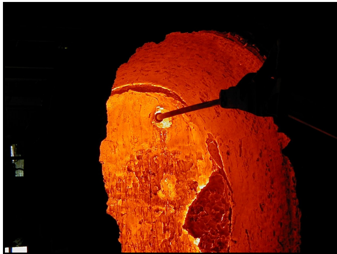
PUSHING PLUG FROM LADLE TAPHOLE
